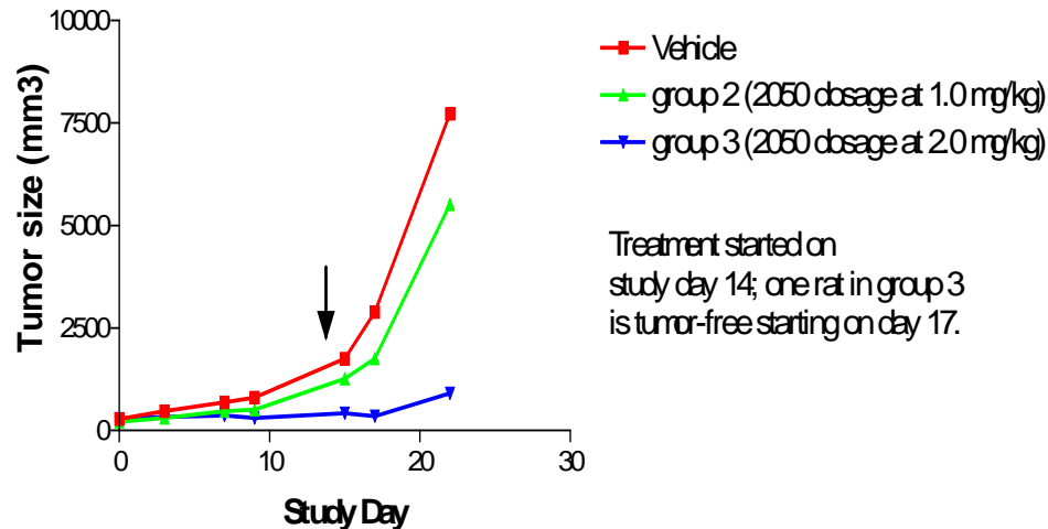
Tumor growth curves of U87 Glioblastoma efficacy study
